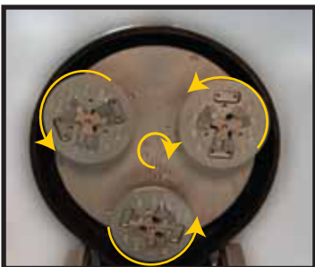
Counter-rotating heads for planetary grinding that contours to the surface.
